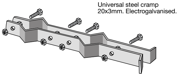
Electrogalvanised guard steel clamp. Appropriate for poles of \varnothing 25 ÷ 40 mm.
